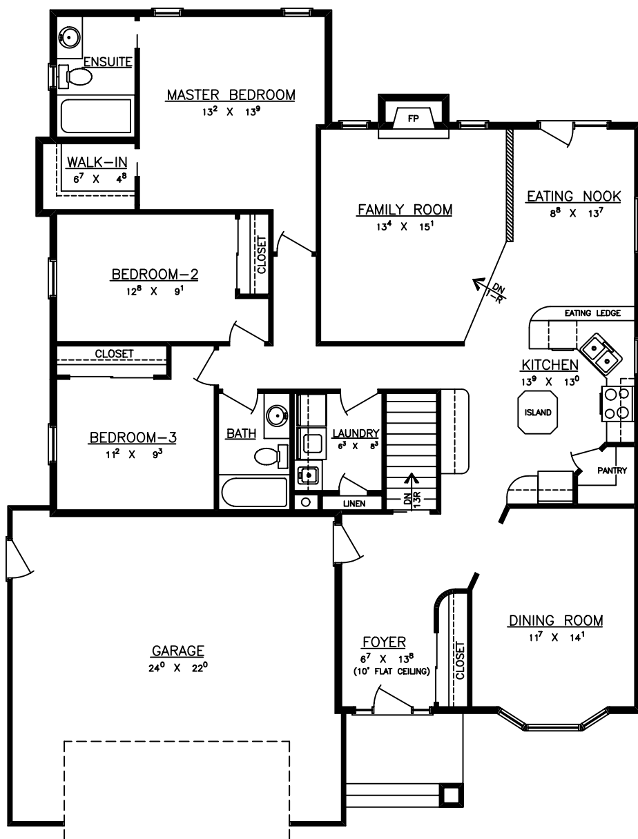
FLOOR PLAN
